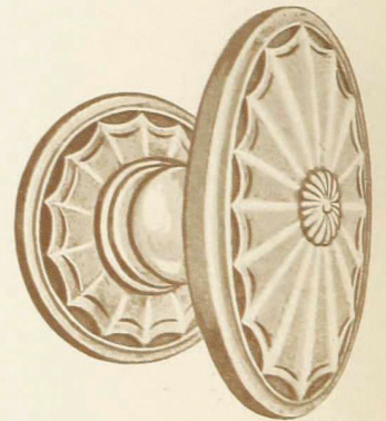
4131 Knob 2\frac{5}{8} \times 1\frac{1}{2} in. 4132 Knob 2\frac{1}{4} \times 1\frac{3}{8} in. 3054 Rose 1\frac{7}{8} in. diam.
